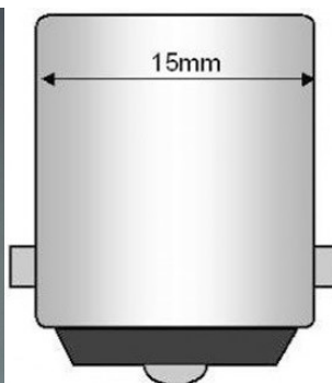
BA15D (1142) Dual Contact Bayonet
