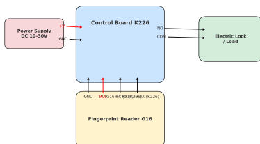
Wiring Diagram - K226 with Fingerprint Reader G16
