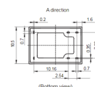
PCB Layout (Bottom view)
