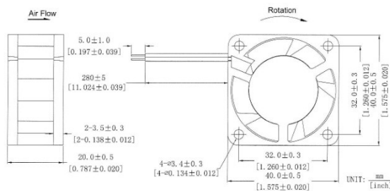
DIMENSIONS DRAWING
