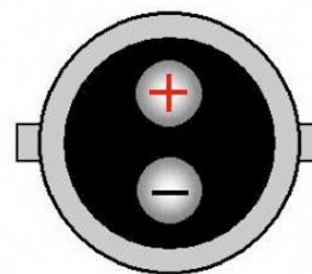
BA15D (1142) Dual Contact Bayonet
