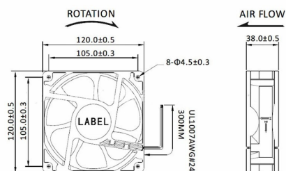
Dimensions Drawing(Unit:mm)
