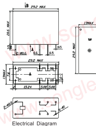
Physical installation diagram
