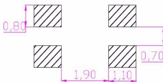
Recommended Soldering Pad Dimensions
