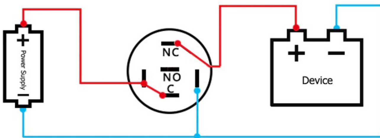
BACKLIGHT ALWAYS ACTIVE, Contact - NC
