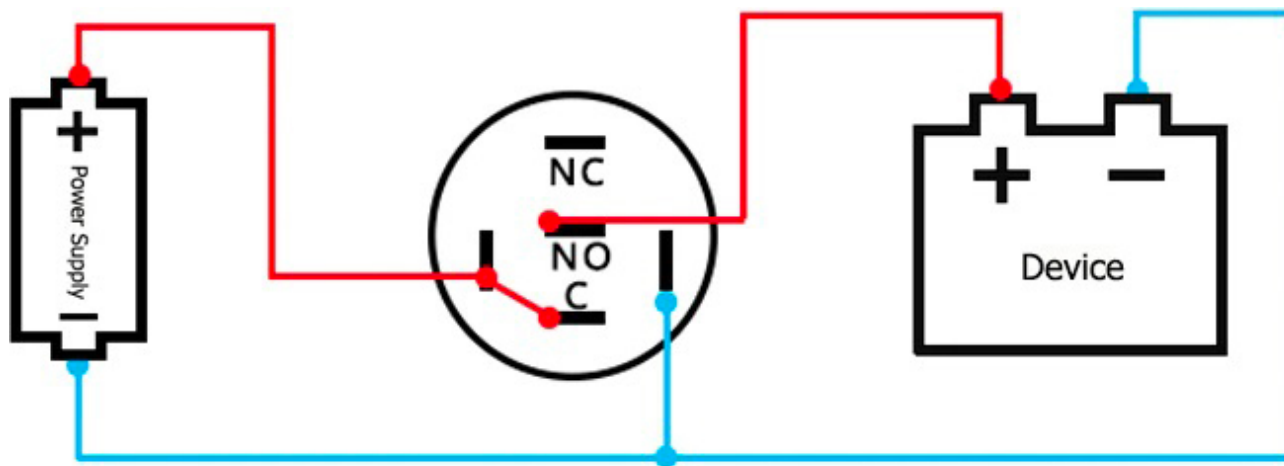
BACKLIGHT STILL ACTIVE, Contact - NO
