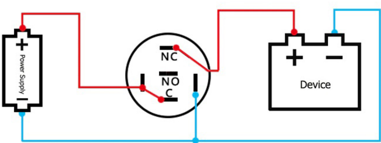
BACKLIGHT ALWAYS ACTIVE, Contact - NC
