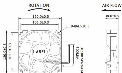
Dimensions Drawing(Unit:mm)
